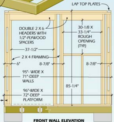
FRONT WALL ELEVATION
