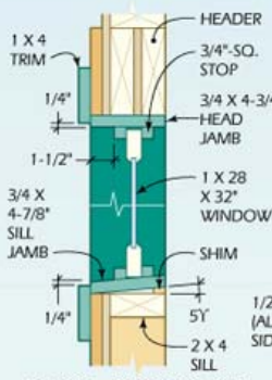
DETAIL 6—WINDOW TRIM
