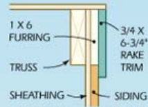
DETAIL 2—RAKE TRIM
