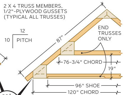
DETAIL 4
