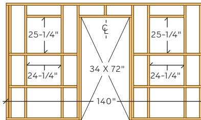
FRONT WALL
