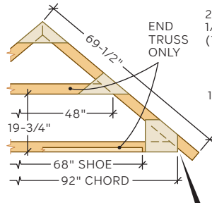
DETAIL 3
