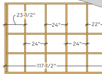
REAR WALL
