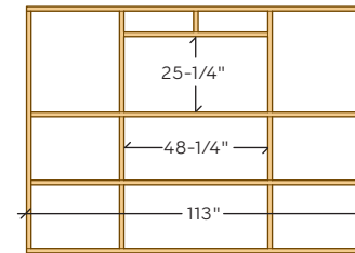
RIGHT WALL
