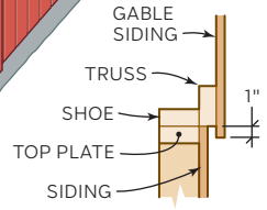
DETAIL 5
